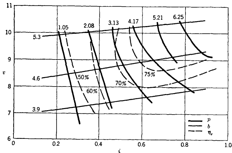
FIG. 10-24a.—Reduced performance chart of SCWC. N \approx 20 ; \sigma = 0.60 ; \mu = 0.50 ; g = 0.85 .
